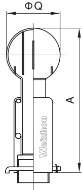
插销式旋转清洗球 Bolted Rotary Cleaning Ball
