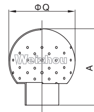
焊接式固定清洗球 Welded Fixed Cleaning Ball
