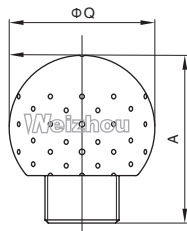
螺纹式固定清洗球 Threaded Fixed Cleaning Ball
