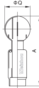
焊接式旋转清洗球 Welded Rotary Cleaning Ball
