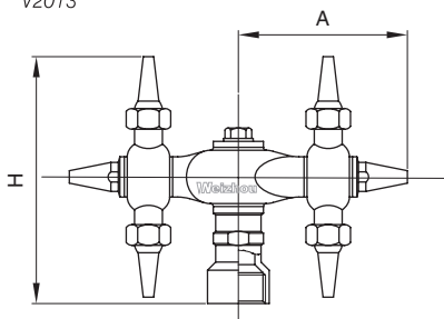
螺纹式旋转清洗球 Threaded Rotary Cleaner
