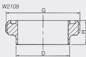
长型螺纹接头 Long male
