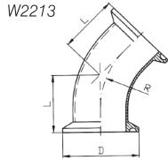
INCH 卡箍弯头 (45°) INCH Clamp Elbow (45°)
