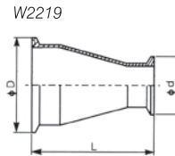
INCH 卡箍式大小头 INCH Clamp Reducer
